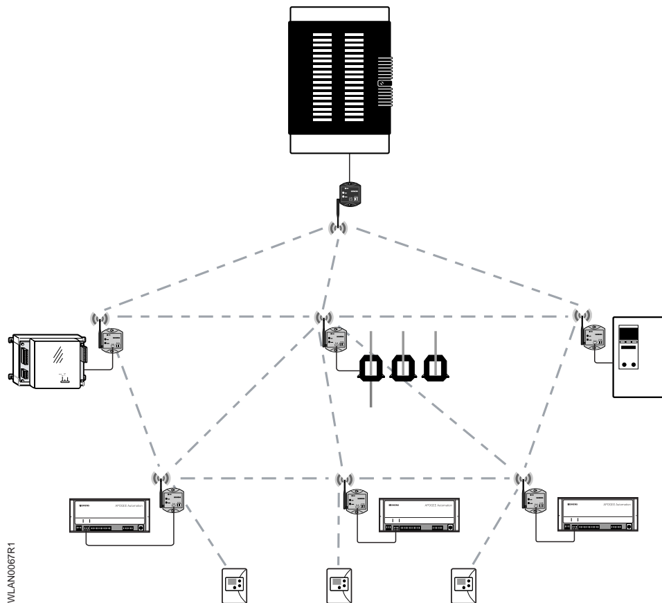
Figure 1. Wireless Field Level Network.
